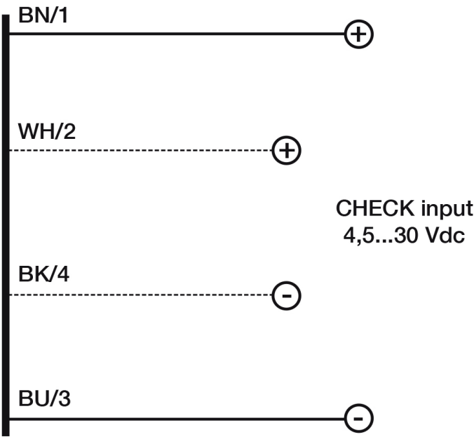
Eletrical diagram
