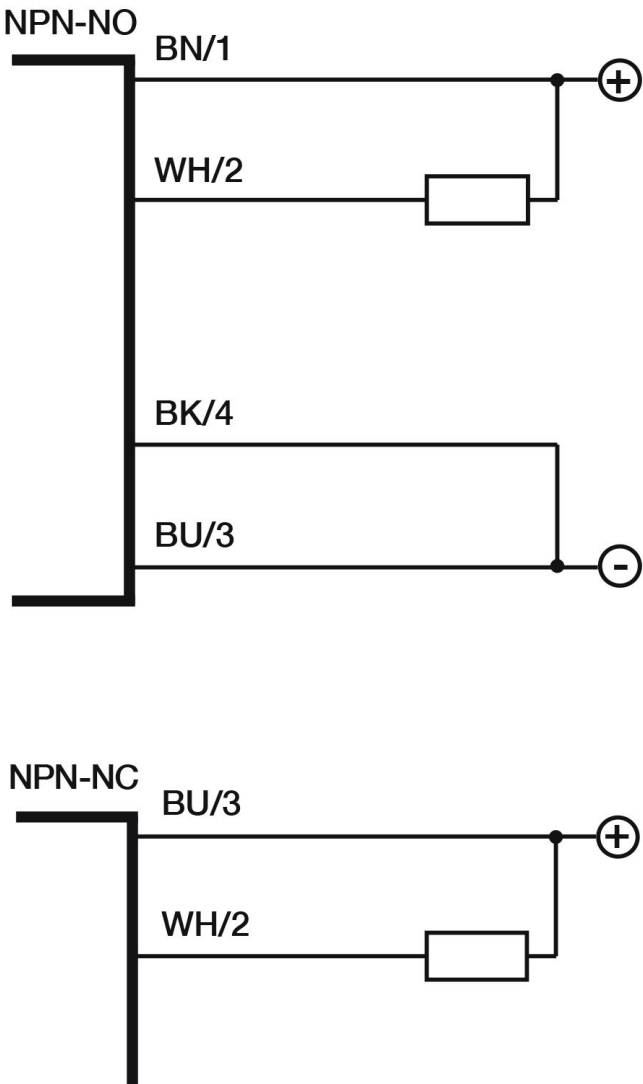
Eletrical diagram
