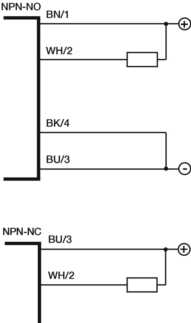
Eletrical diagram
