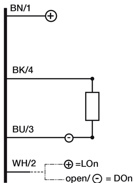
Eletrical diagram
