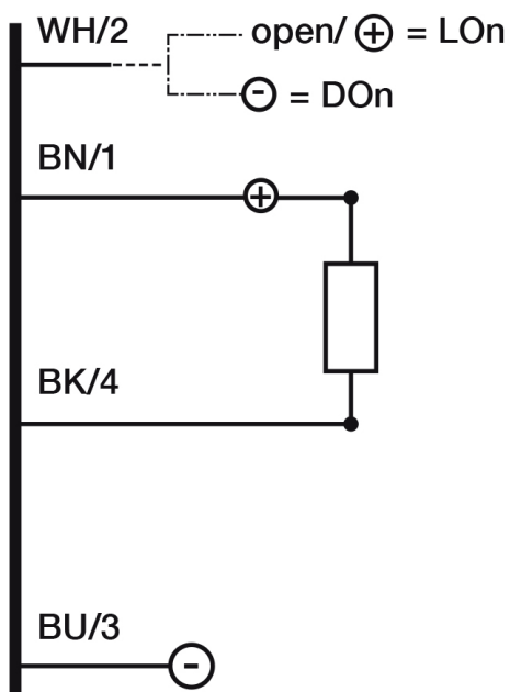
Electrical diagram
