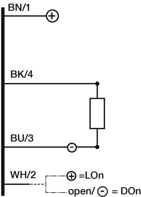
Electrical diagram
