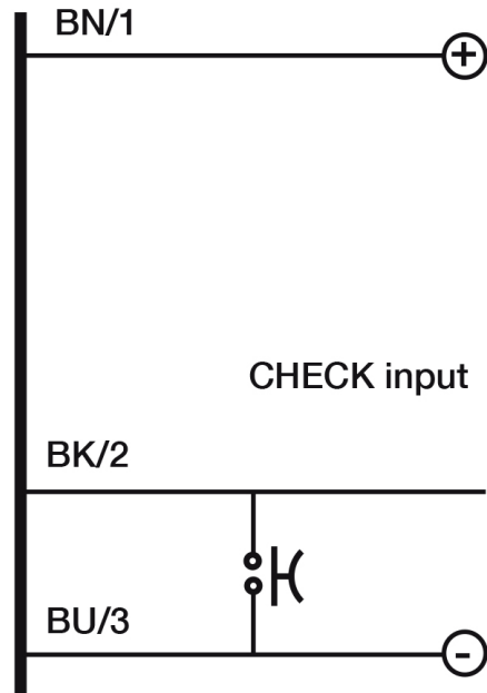
Connector
