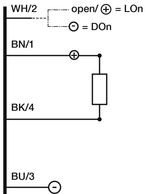
Eletrical diagram
