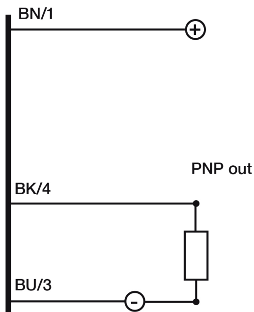
Eletrical diagram
