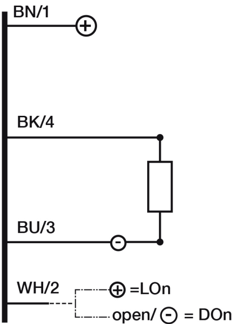
Eletrical diagram
