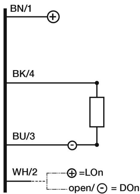
Eletrical diagram
