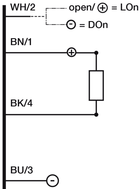
Eletrical diagram
