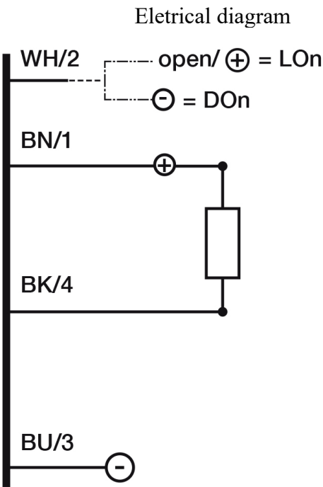
Connector
