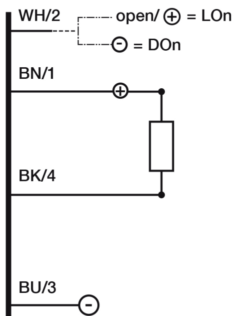
Eletrical diagram
