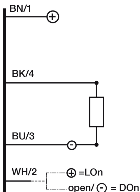
Eletrical diagram
