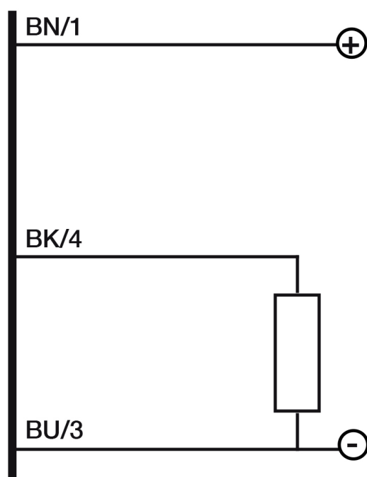
Eletrical diagram
