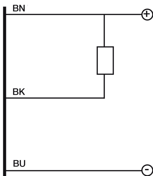
Electrical diagram
