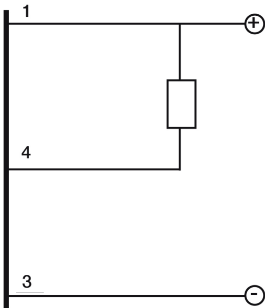
Eletrical diagram
