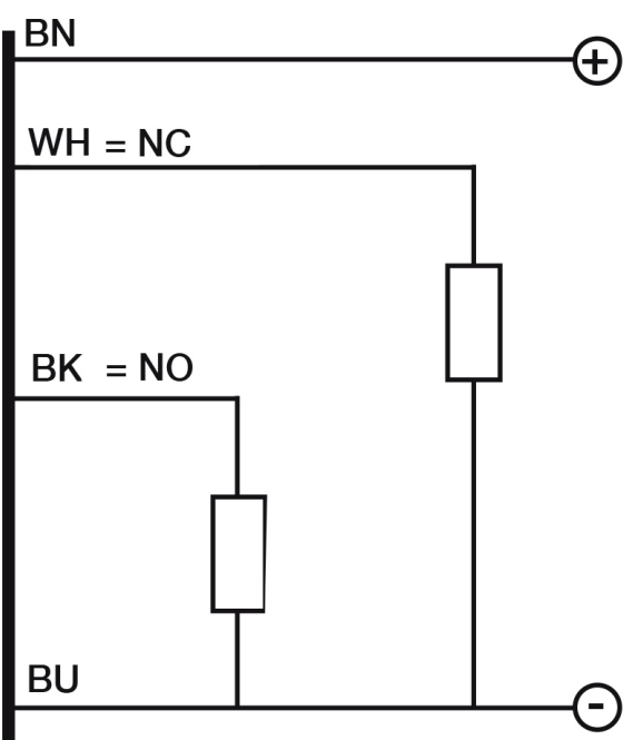
Eletrical diagram
