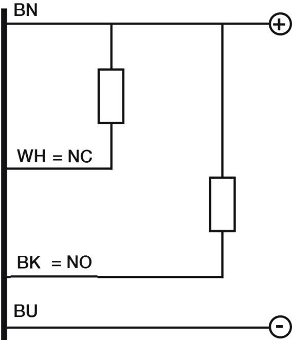
Eletrical diagram
