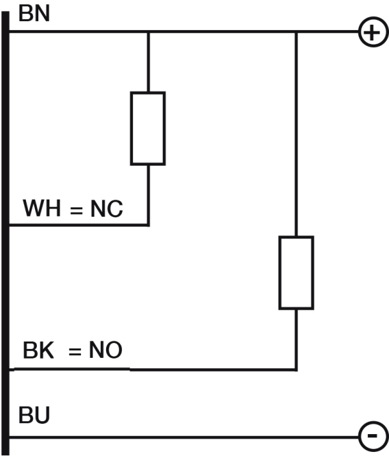
Connector
