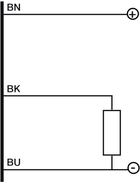
Eletrical diagram
