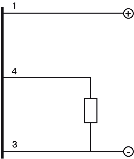
Eletrical diagram
