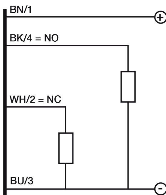
Electrical diagram
