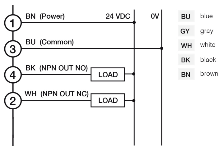
Eletrical diagram
