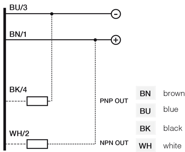
Eletrical diagram
