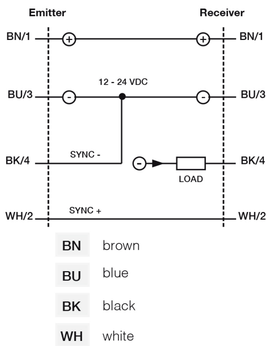
Electrical diagram
