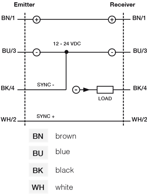
Eletrical diagram
