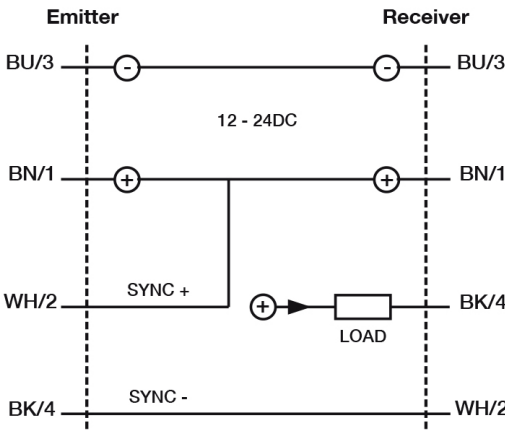
Eletrical diagram
