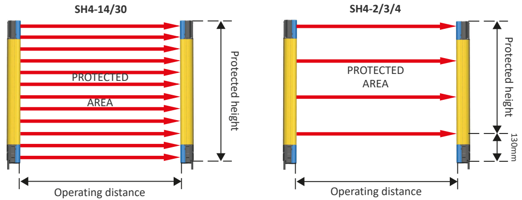
Figure 2: Detection zone
