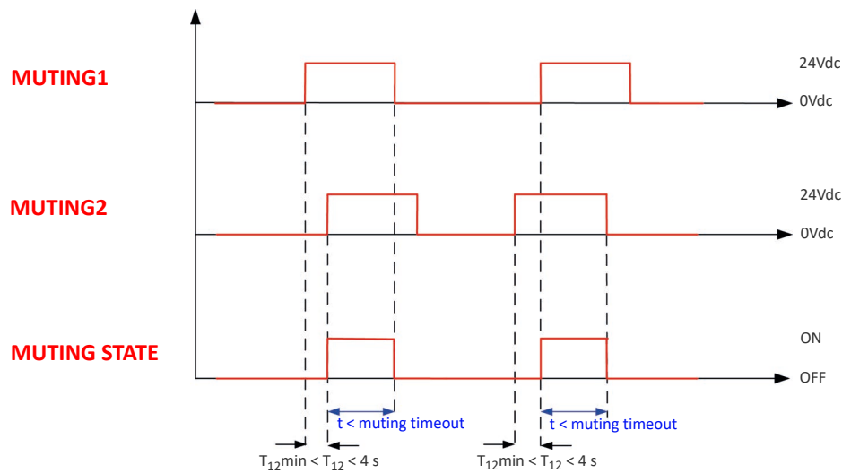
Figure 39: T muting timings
