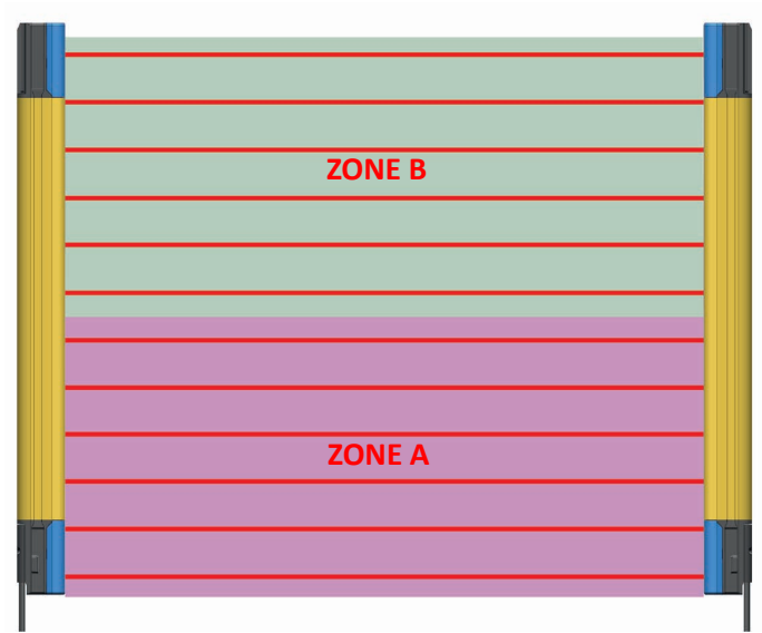
Figure 41: Partial muting
