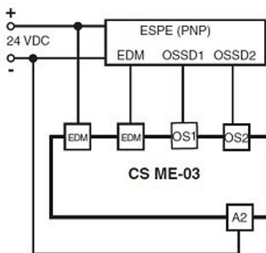
Figure 70 - EDM relay
