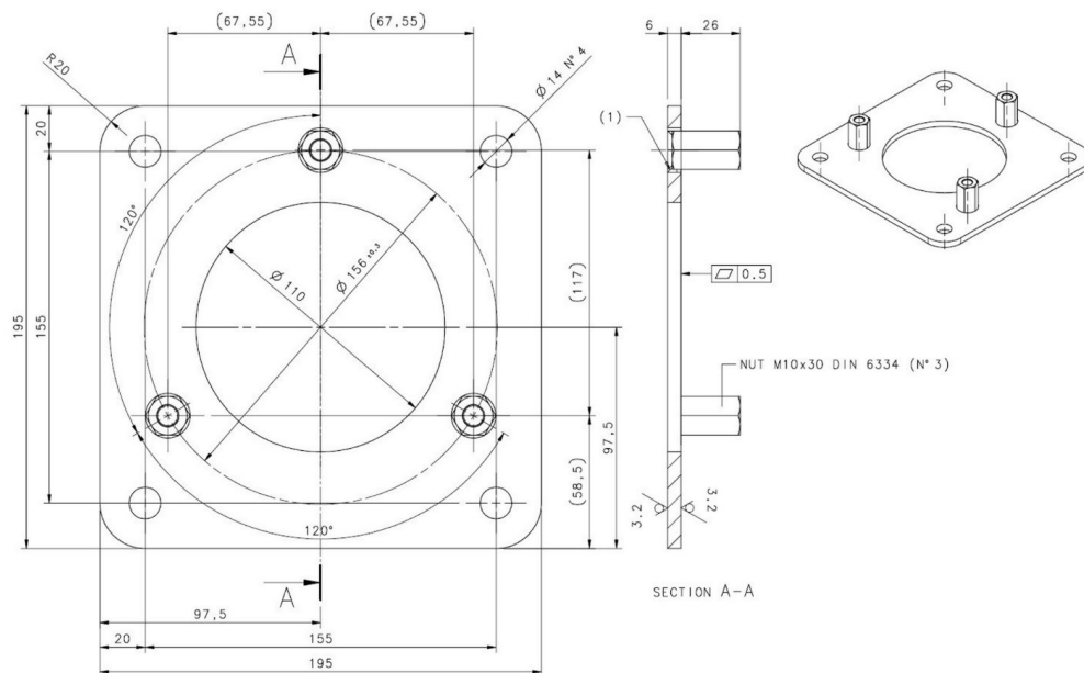
Figure 61 – Plate kit
