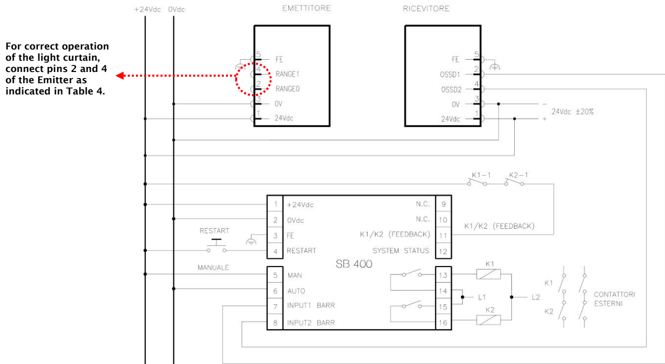
Figure 21 - LS2: Manual operation with SB400 module
