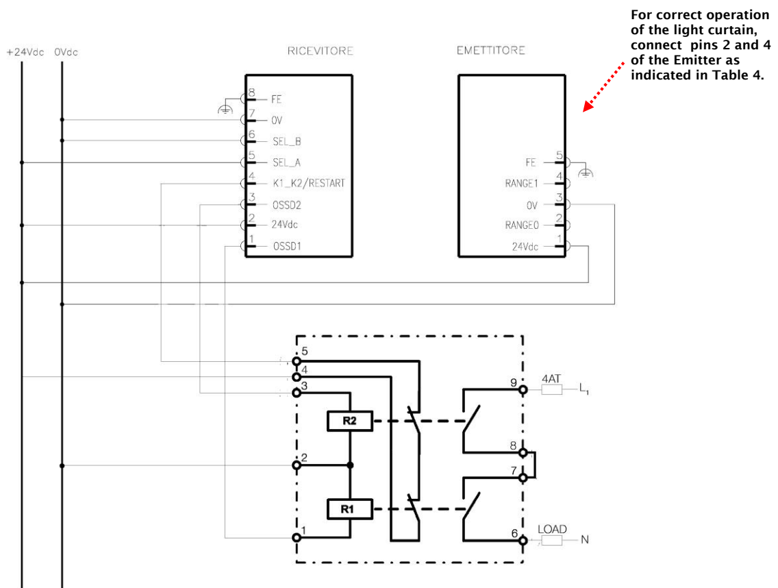
Figure 22 – LS2: Automatic operation with SB300 module
