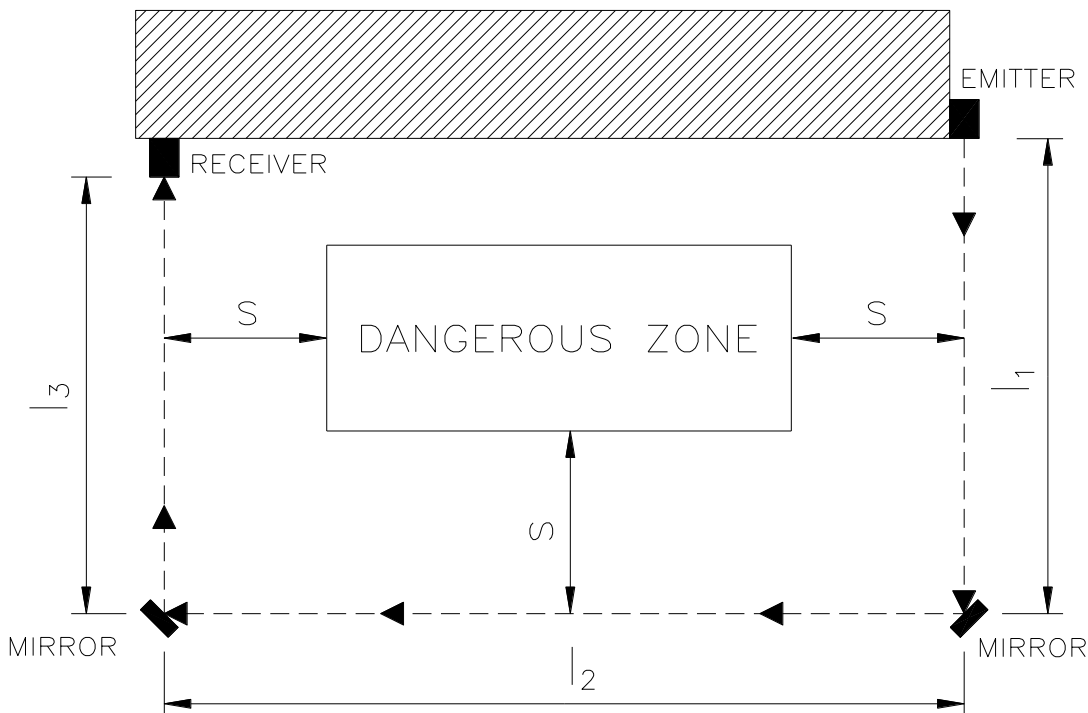
Figure 7 – Deflecting mirrors
