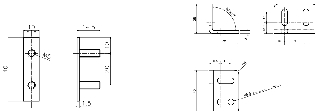
Figure 28 - ST204 inserts and fastening brackets (provided)
