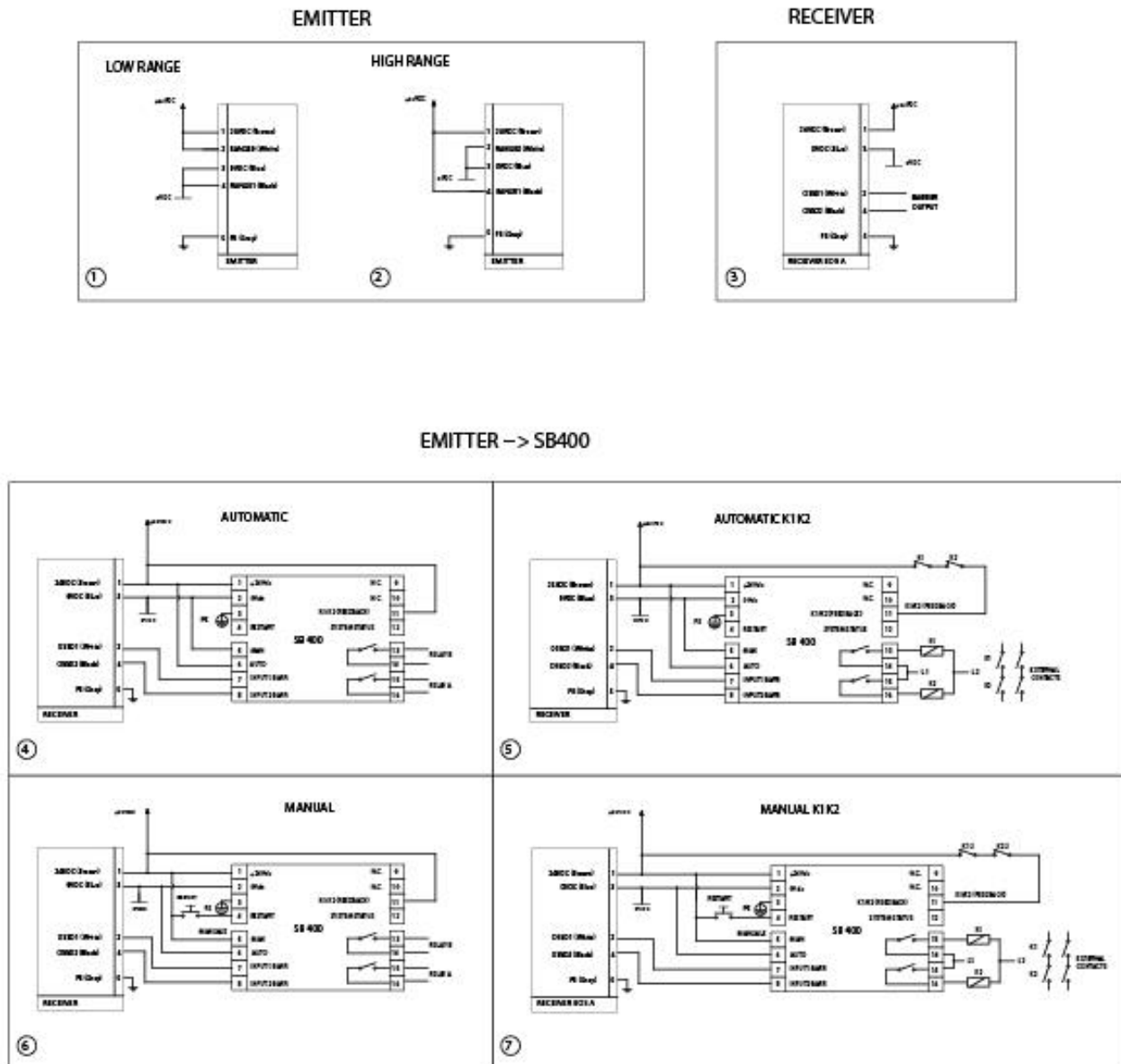
Figure 24 - LS2R/**-***: Connection examples
