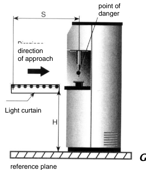
Figure 15 - Horizontal positioning
