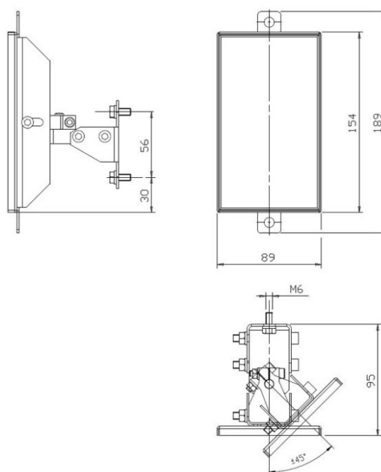
Figure 7 - SG-DM 150 (mm)
