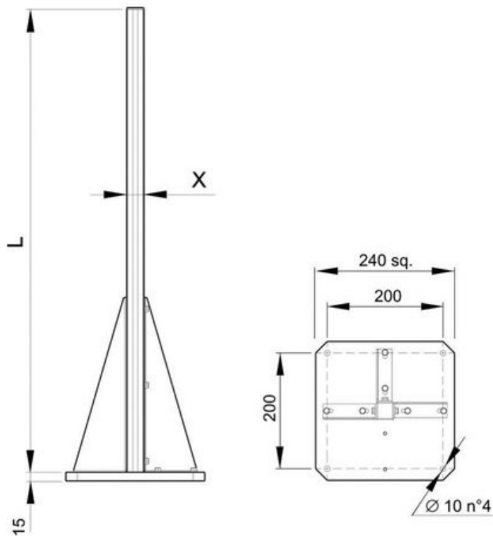
Figure 5 - Dimensions (mm)
