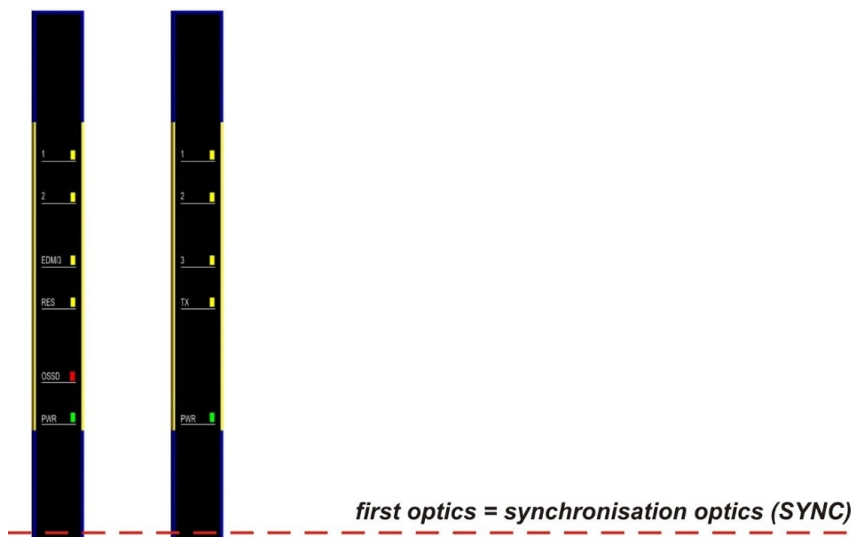
Figure 1 - Synchronization Optics
