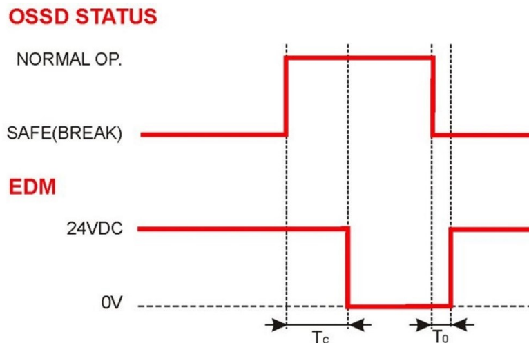
Figure 6 - EDM timings
