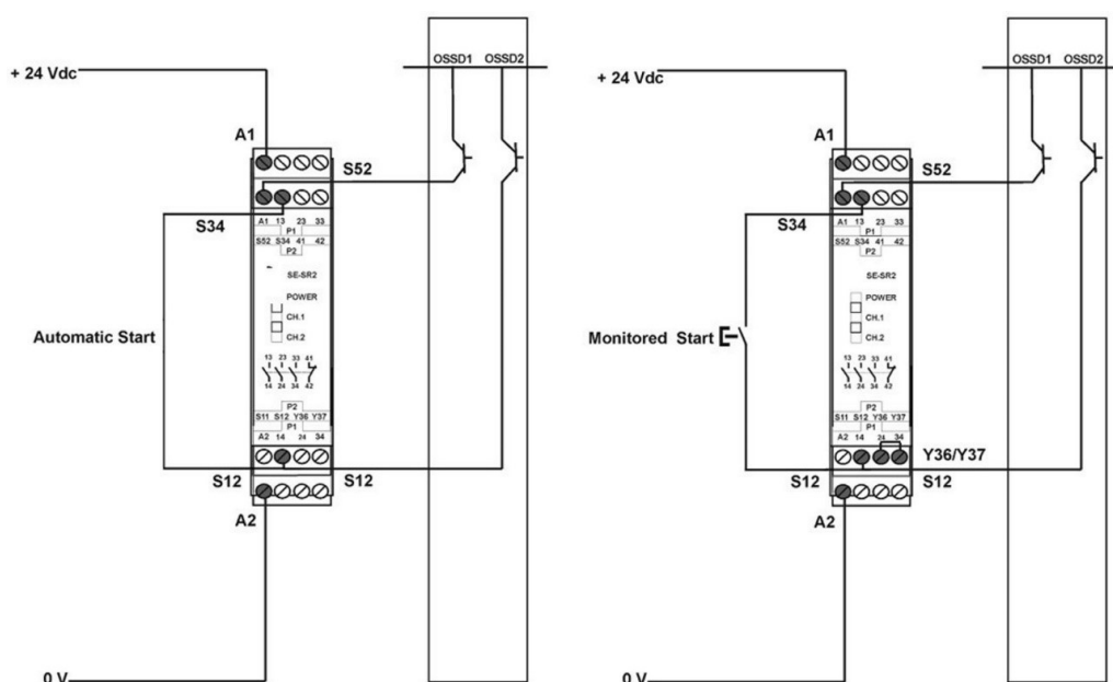
Figure 10 - Safety relay
