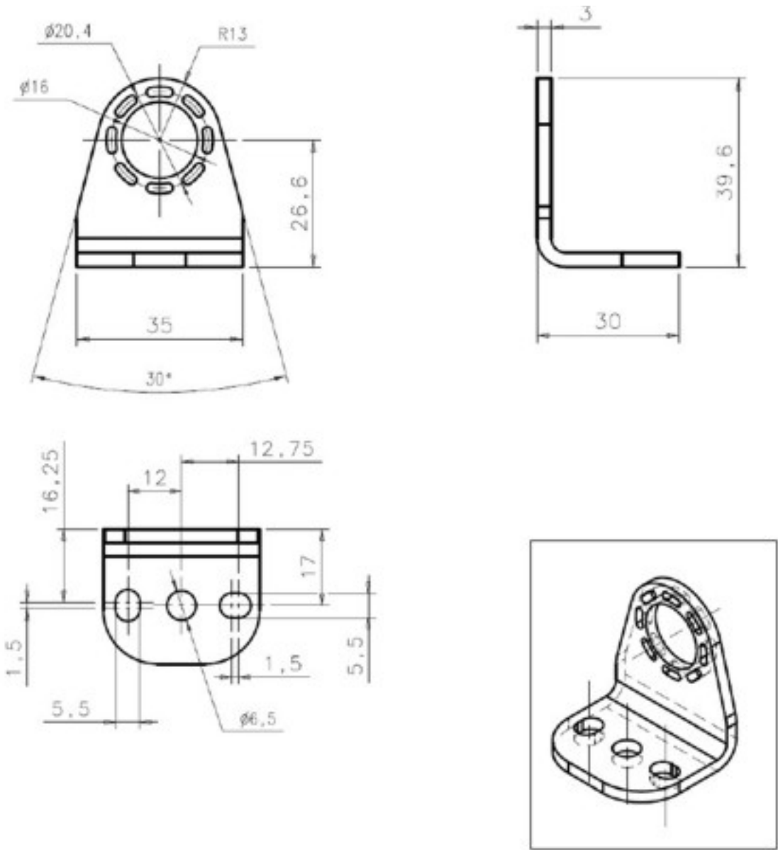
Fig 54 - Dimensions (mm)
