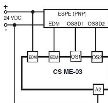
Fig 71 - EDM Relay
