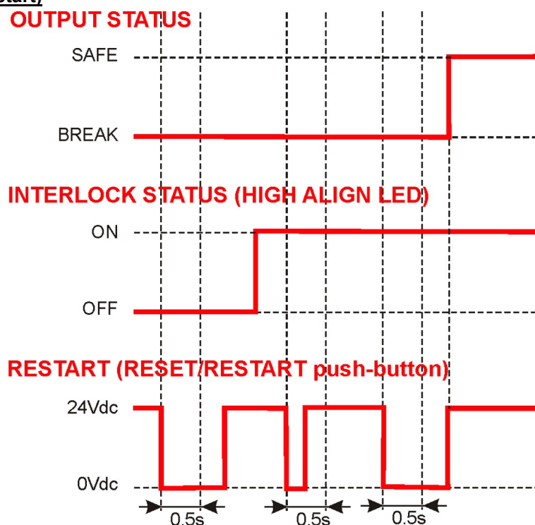
Fig 35 - Time chart (Manual Restart)
