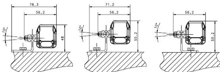
Fig 46 - Angled fixing bracket + Orientable support
