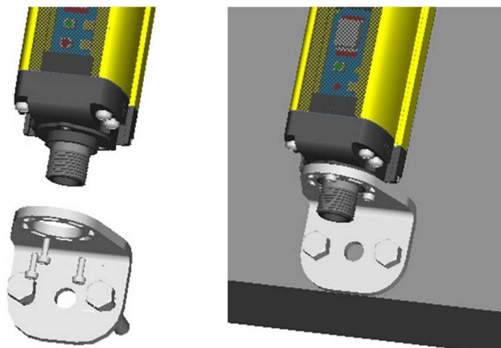
Fig 22 - Rotating brackets
