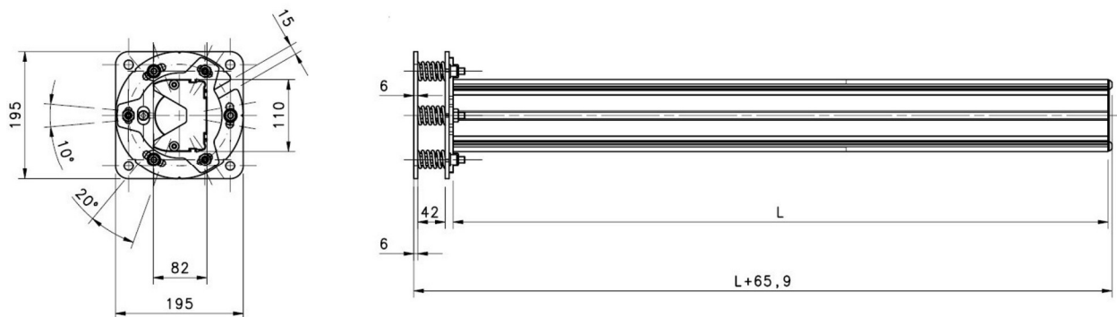
Fig 58 - Mounting
