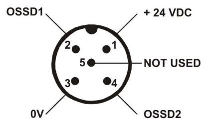
Fig 25 - Receiver
