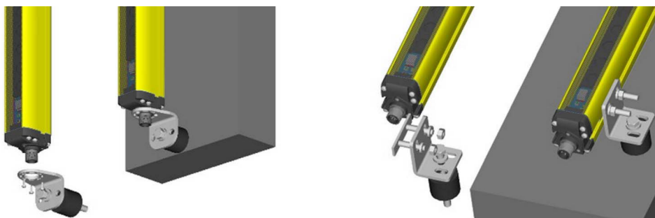
Fig 23 - Fixing brackets
