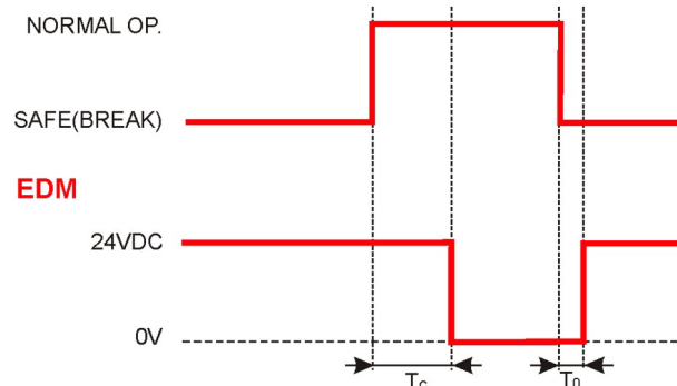
Fig 39 - OSSD status
