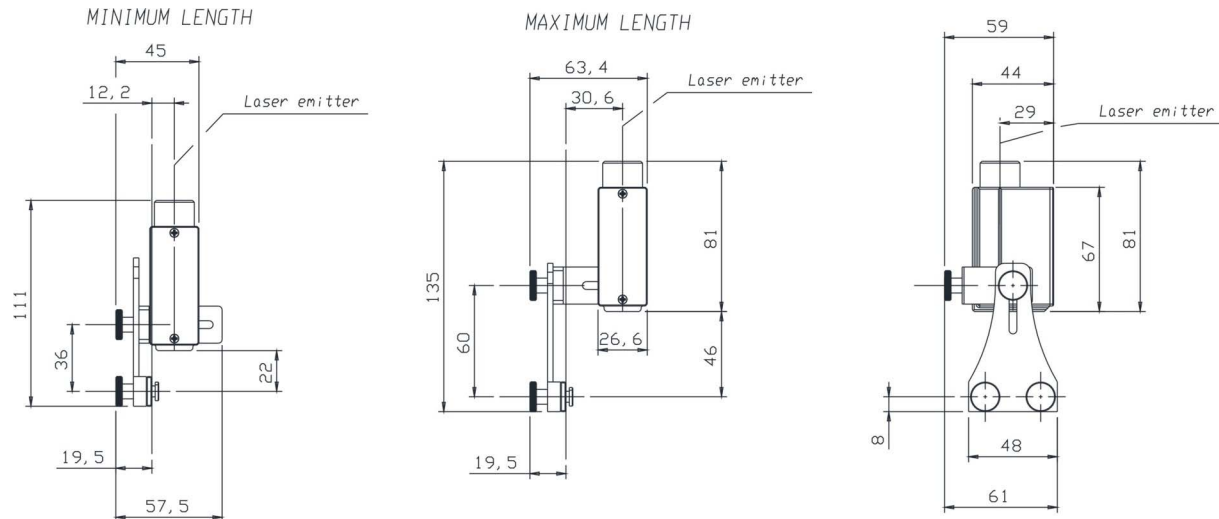
Fig 68 - Dimensions (mm)
