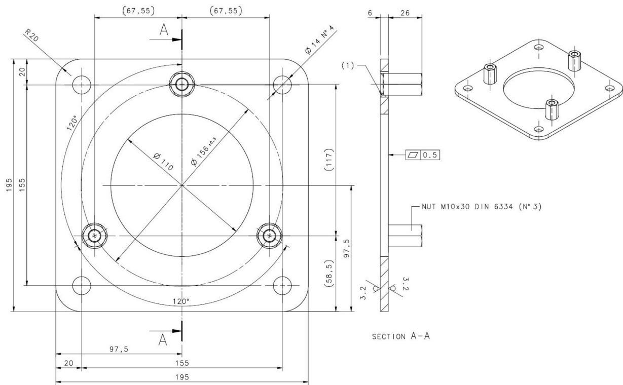
Fig 57 - Dimensions (mm)
