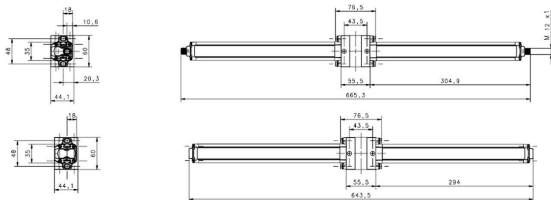
Fig 112 - Active/Passive arms T
