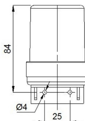
Fig 105 - Lamp LMS-2
