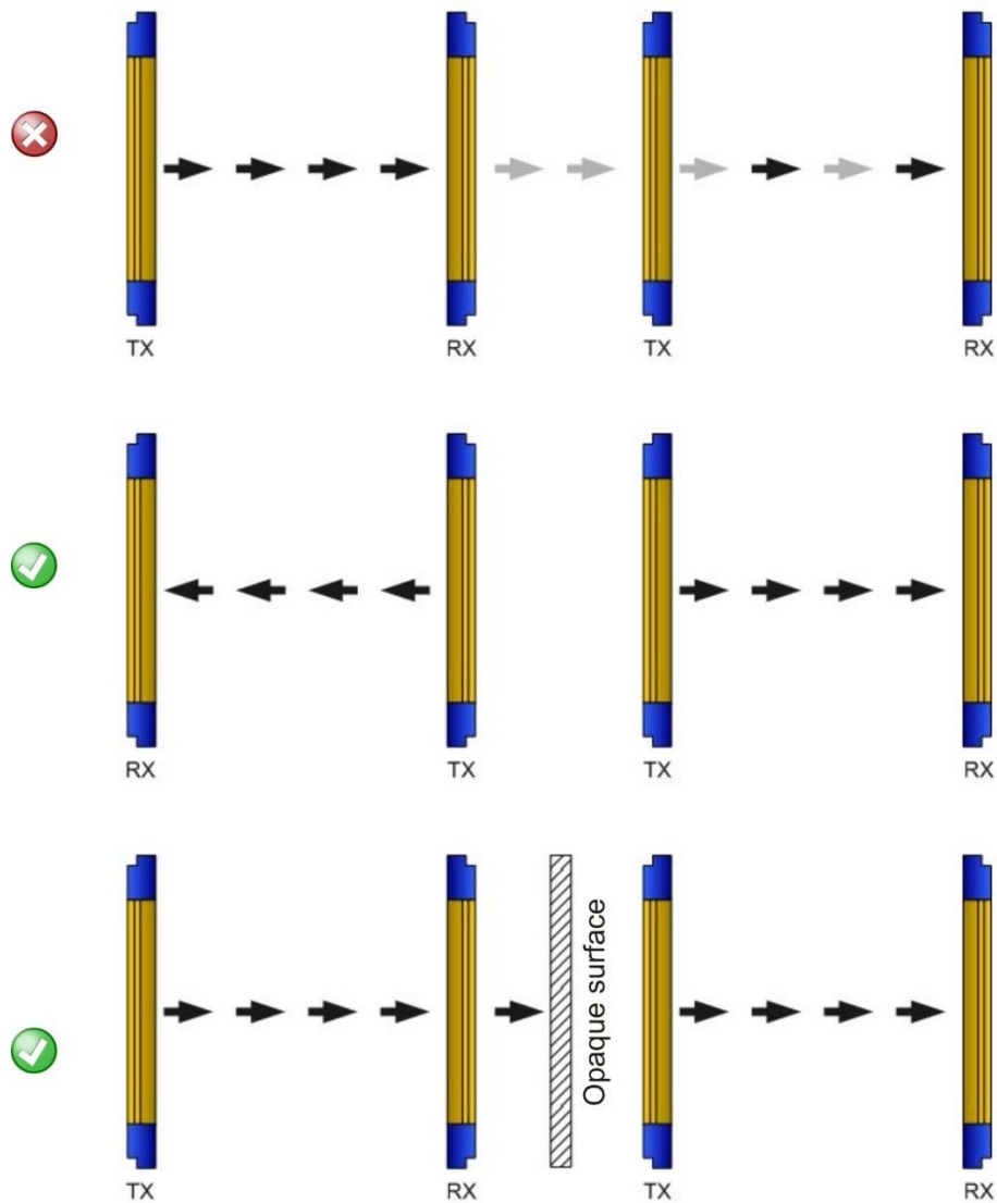
Fig 17 - Recommended positioning for homologous devices
