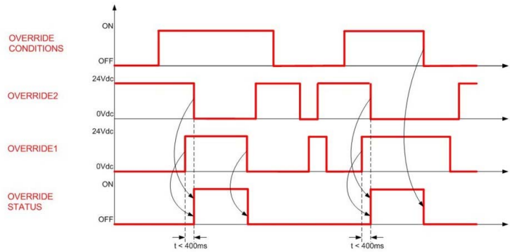
Fig 68 - Override timings (level trigger)
