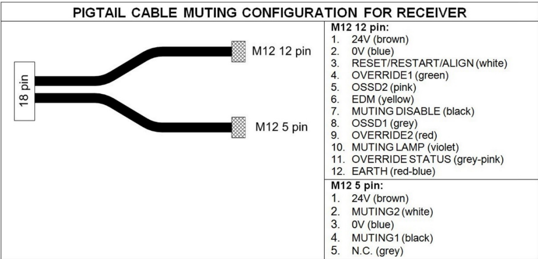
Fig 25 - Pigtail cable - Muting configuration for receiver RX (CS-R1-75-B-002)
