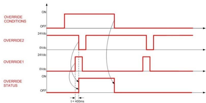
Fig 69 - Override timings (edge trigger)
