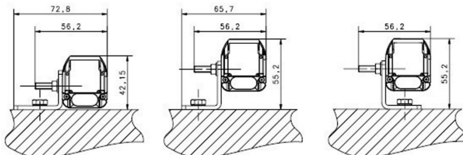
Fig 80 - Angled fixing bracket
