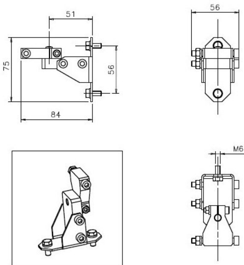
Fig 96 - Mounting kit
