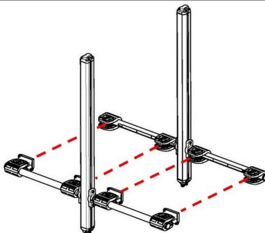
Fig 116 - T-MUTING
