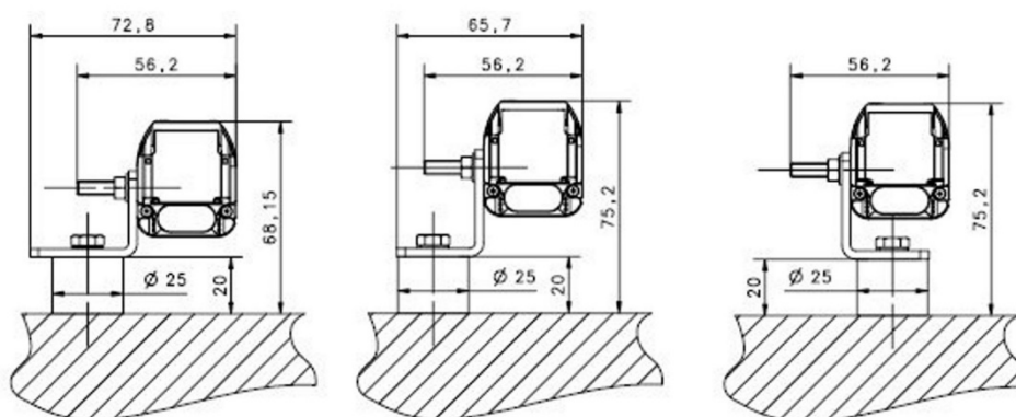
Fig 82 - Angled fixing bracket + Antivibration support
