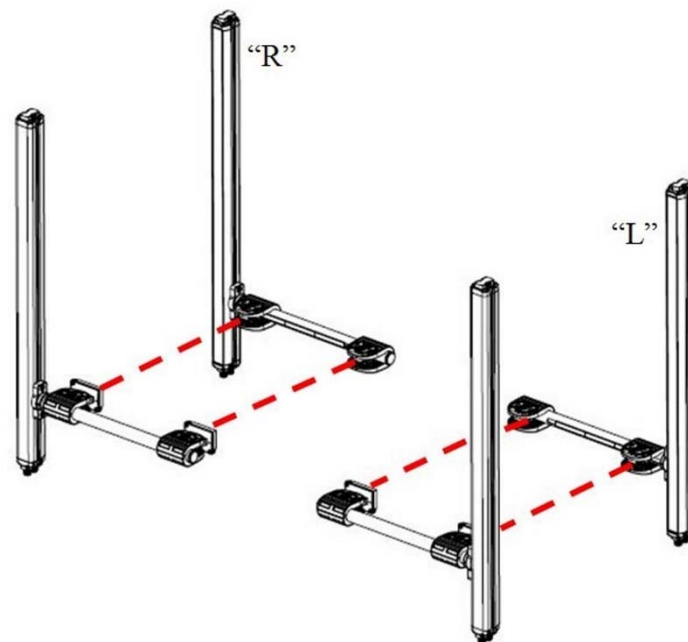
Fig 115 - L-MUTING
