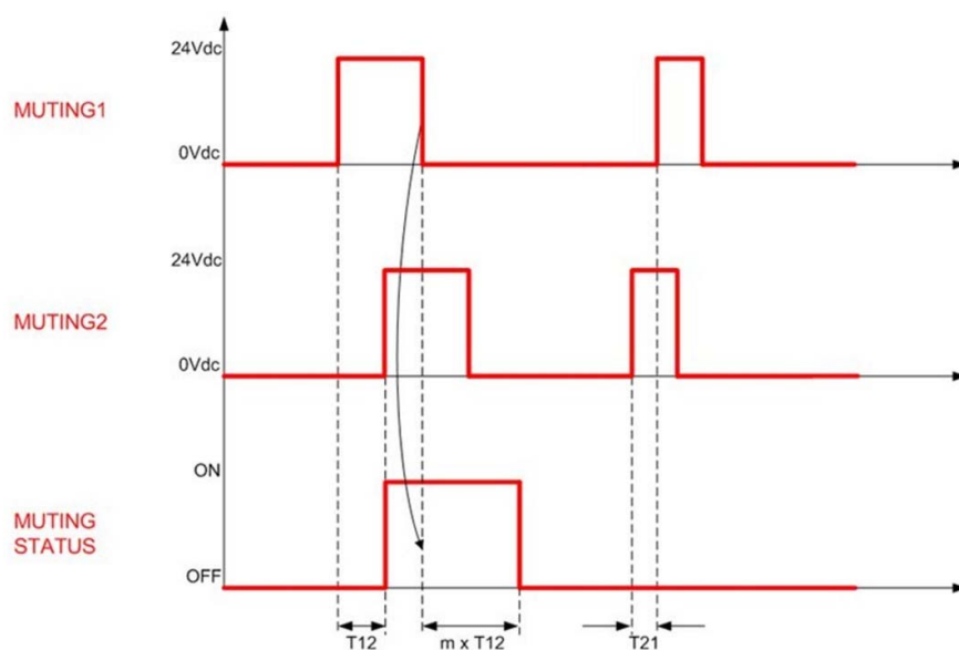
Fig 60 - Muting L timings
