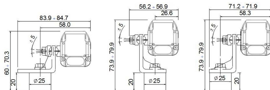
Fig 88 - Angled fixing bracket + Orientable support + Antivibration support
