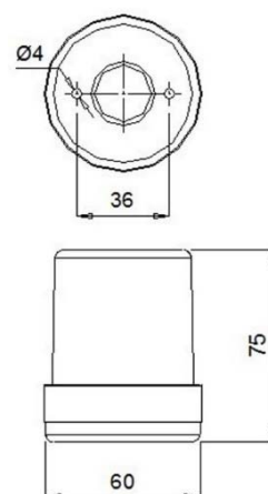
Fig 105 - Lamp LMS-2
