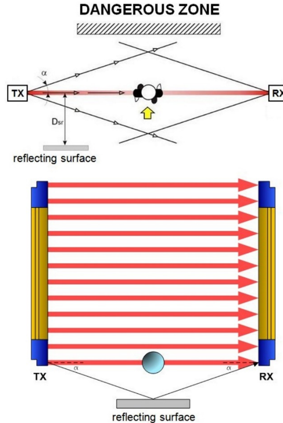
Fig 13 - Distance from reflecting surfaces
