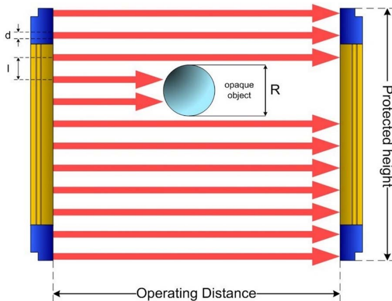
Fig 2 - Detection capability
