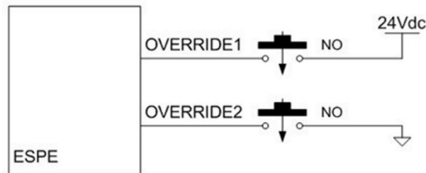
Fig 66 - Override connection
