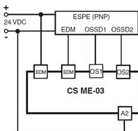
Fig 103 - EDM Relay
