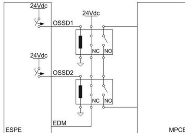
Fig 48 - PNP configuration
