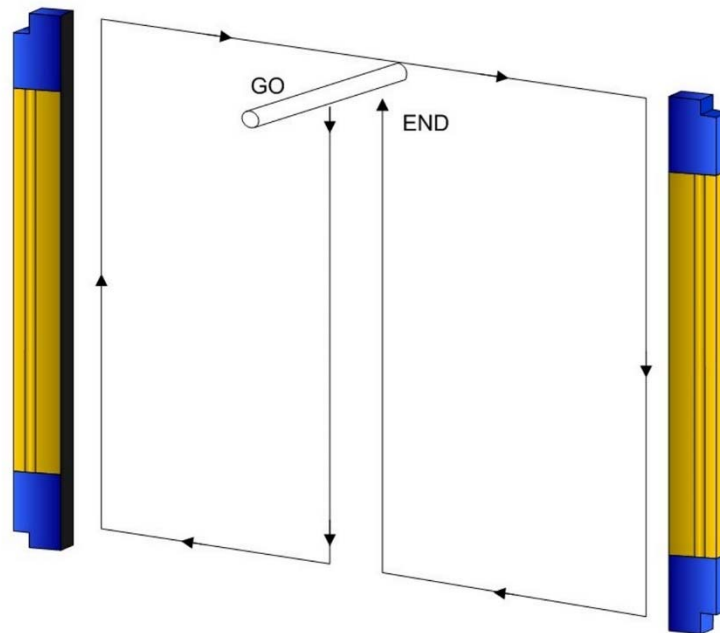
Fig 20 - Path of the test piece
