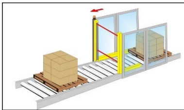
Fig 54 - L-shaped version with integrated Muting sensors for unidirectional Muting
