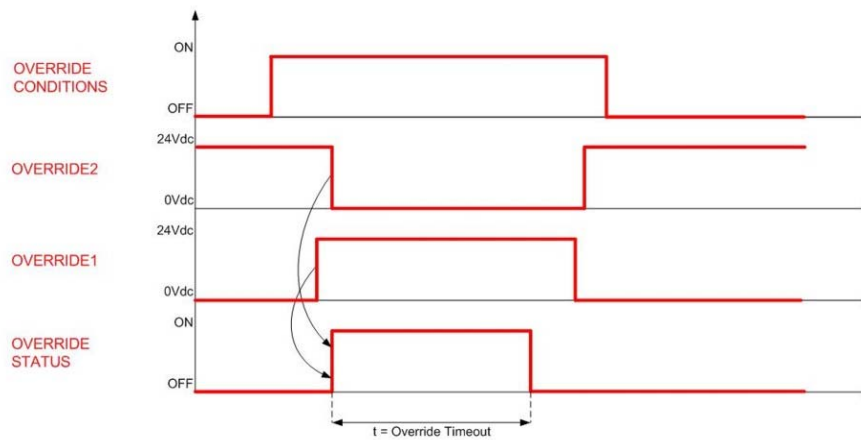
Fig 71 - Override timeout timings
