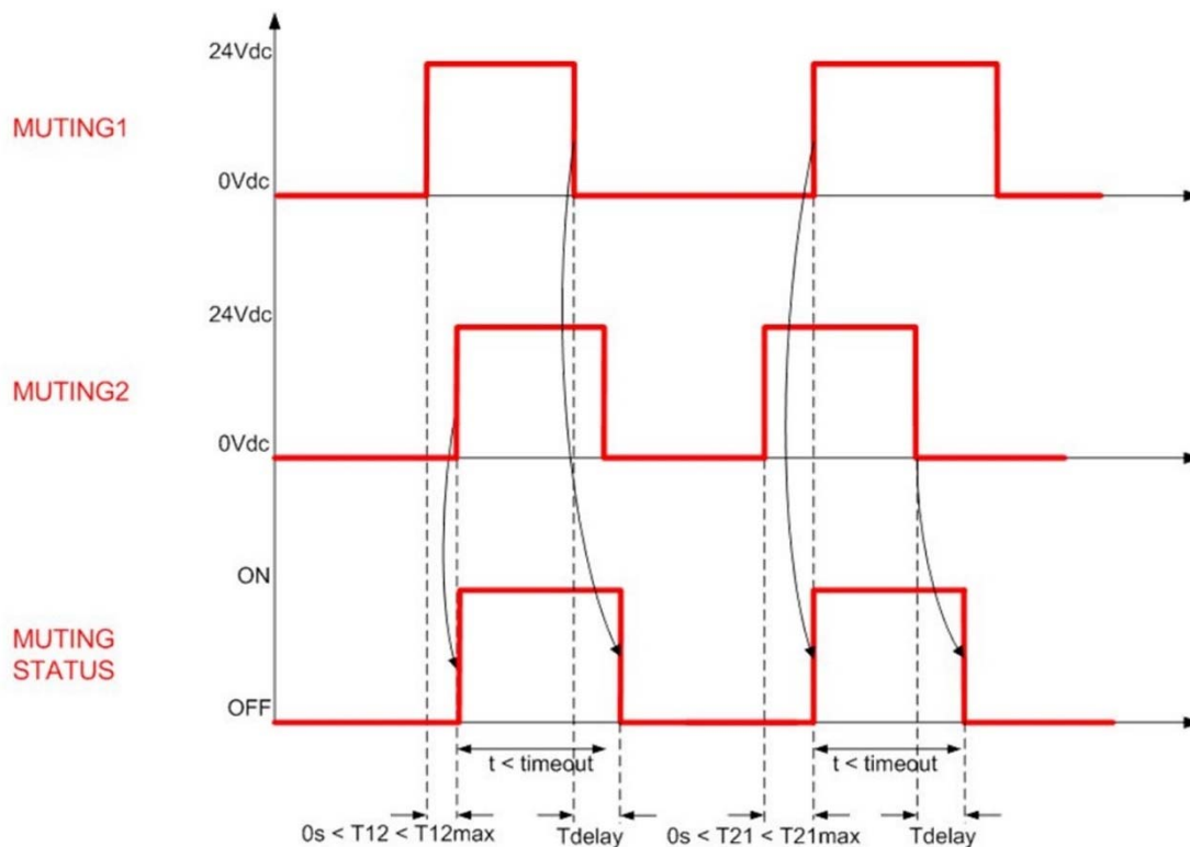
Fig 58 - T Muting timings
