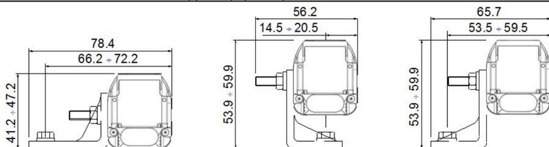
Fig 85 - Angled fixing bracket
