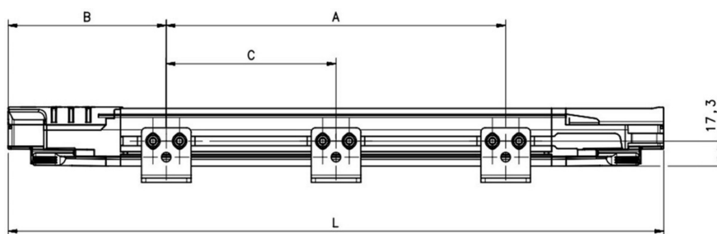
Fig 23 - Light curtain dimensions
