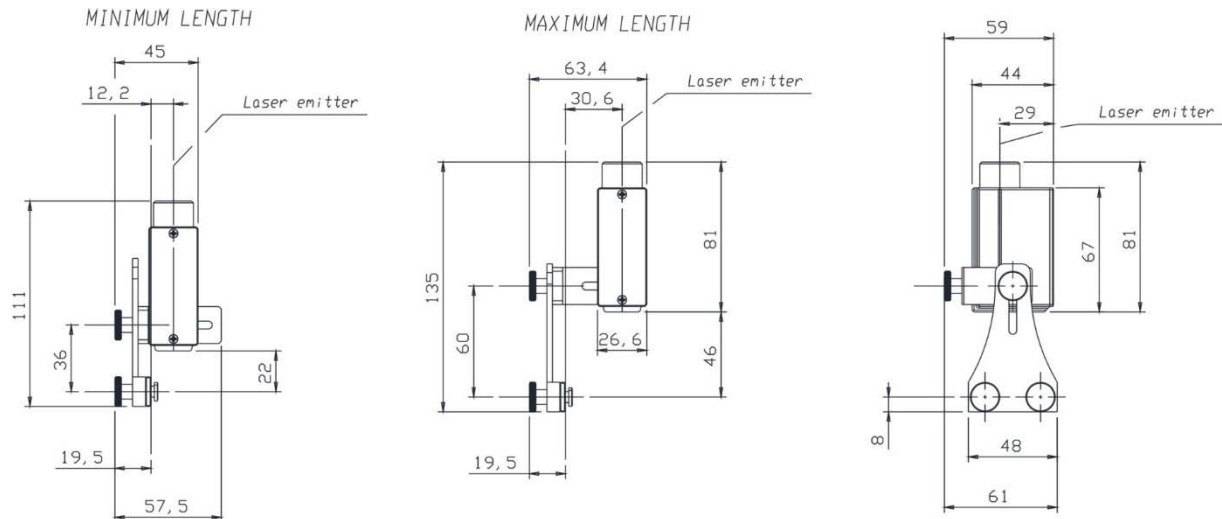
Fig 100 - Dimensions (mm)
