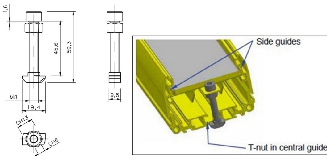
Fig 97 - Mounting kit
