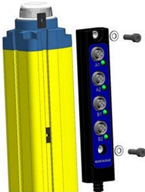
Fig 121 - Connection box
