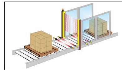
Fig 56 - Linear version with external Muting sensors
