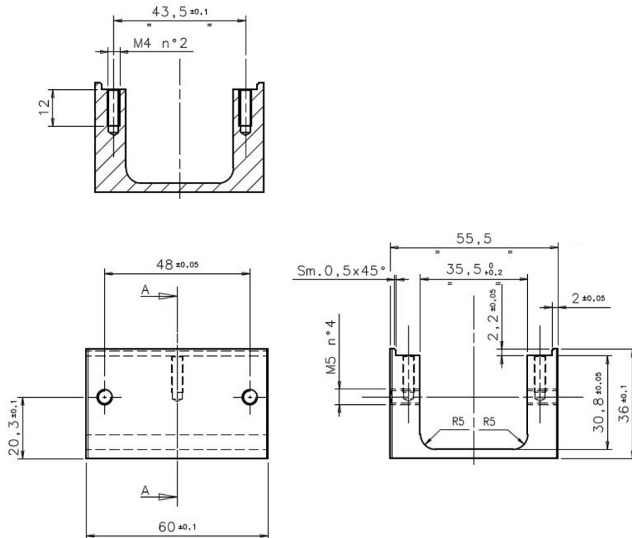
Fig 110 - Mounting bracket
