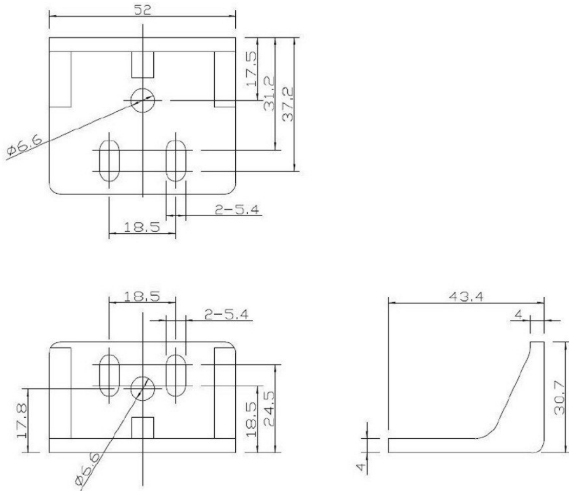
Fig 84 - ST-KPxMP
