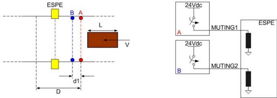
Fig 61 - Muting L connection
