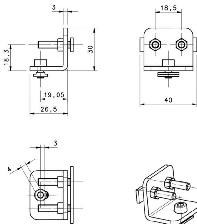
Fig 90 - Fixing kit
