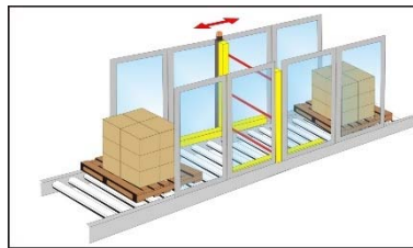
Fig 55 - T-shaped version with integrated Muting sensors for bidirectional Muting
