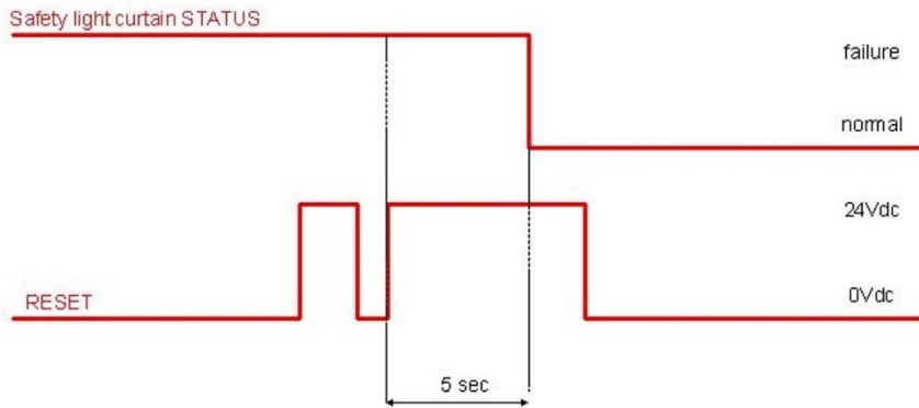
Fig 47 - Reset timings
