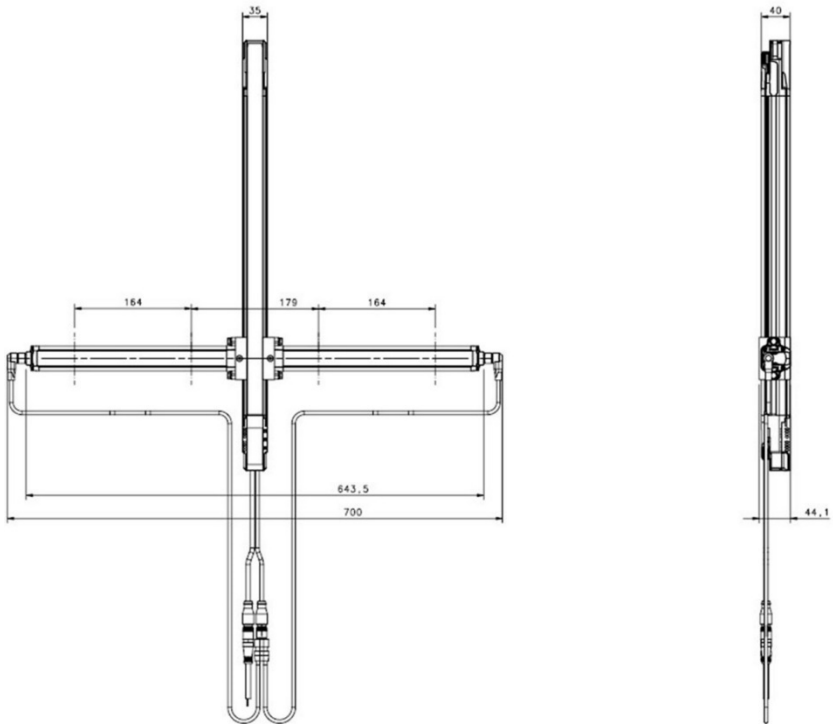
Fig 114 - Light curtain + Active/Passive arms T
