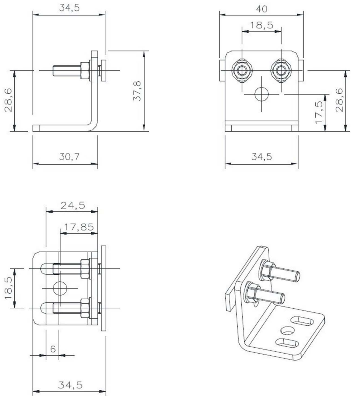
Fig 76 - Dimensions (mm)
