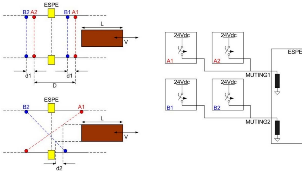
Fig 59 - Muting T connection
