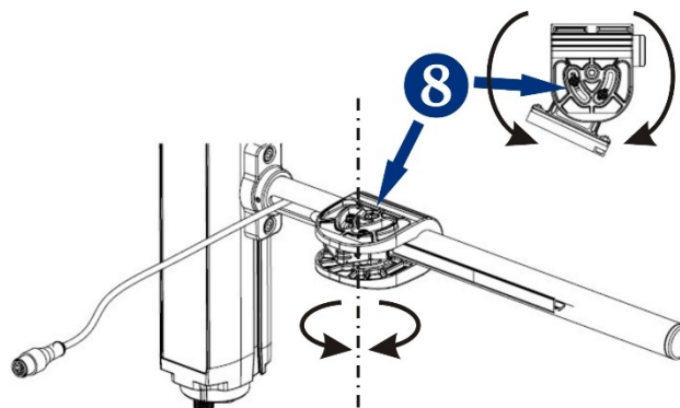
Fig 120 - Phase 3
