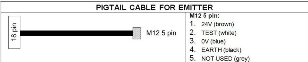
Fig 26 - Pigtail cable - configuration for emitter TX (CS-G1-50-B-002)
