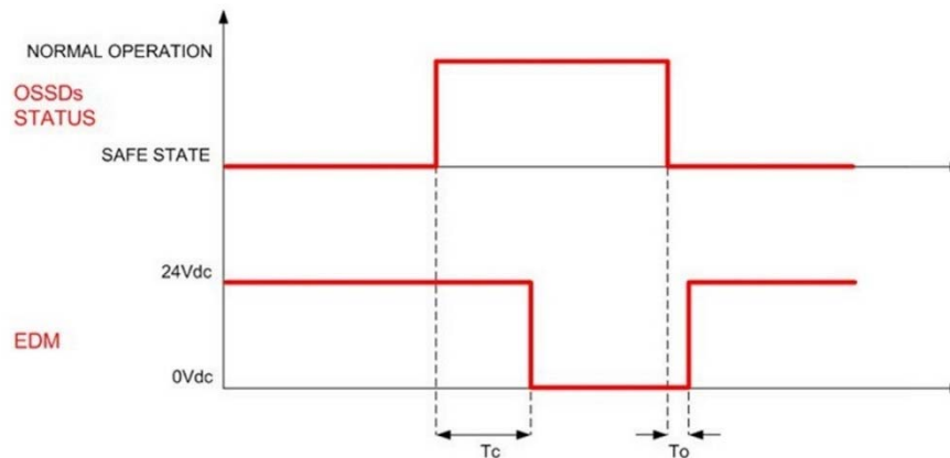
Fig 49 - EDM timings (PNP configuration)
