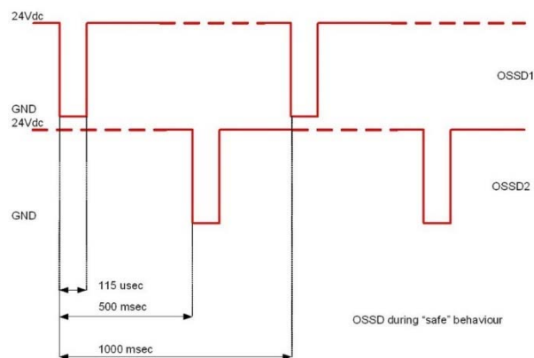
Fig 33 - Behaviour of OSSDs
