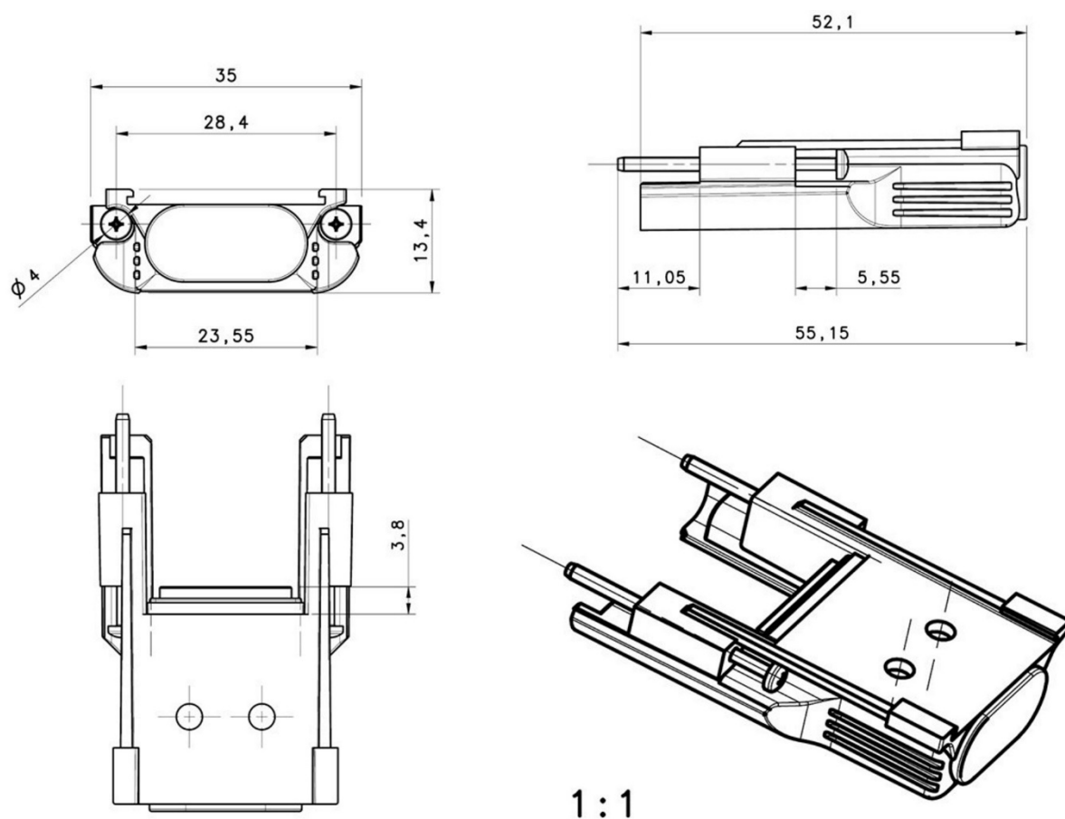
Fig 77 - Dimensions (mm)
