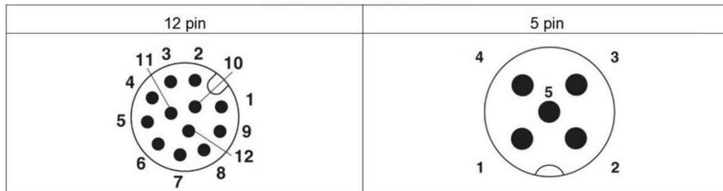
Fig 27 - M12 Connectors pinout
