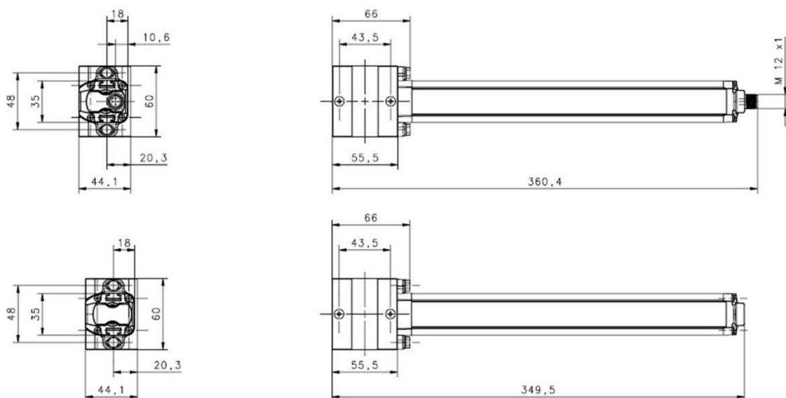
Fig 111 - Active/Passive arms L
