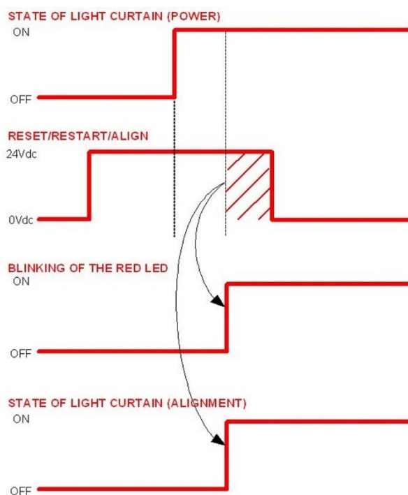
Fig 35 - Alignment timings
