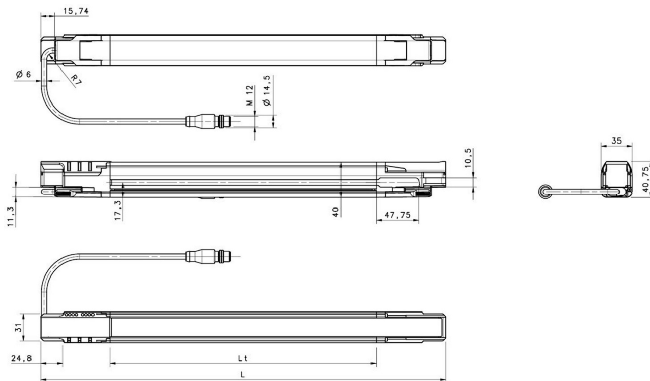
Fig 75 - Overall dimensions (mm)
