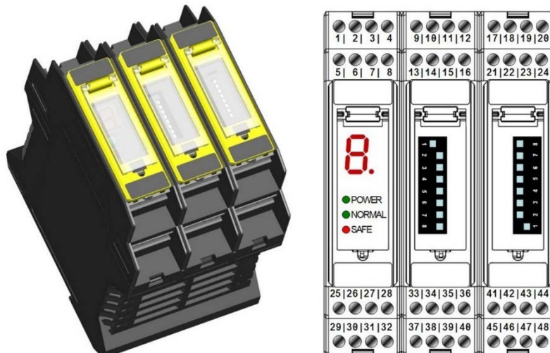
Fig 126 - SG-BWS-T4-MT Safety control unit
