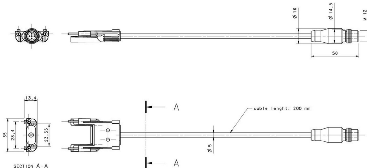
Fig 98 - TX - Pigtail cable
