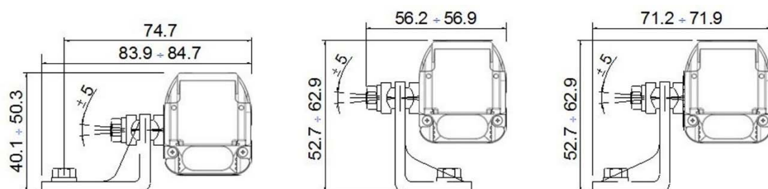
Fig 86 - Angled fixing bracket + Orientable support
