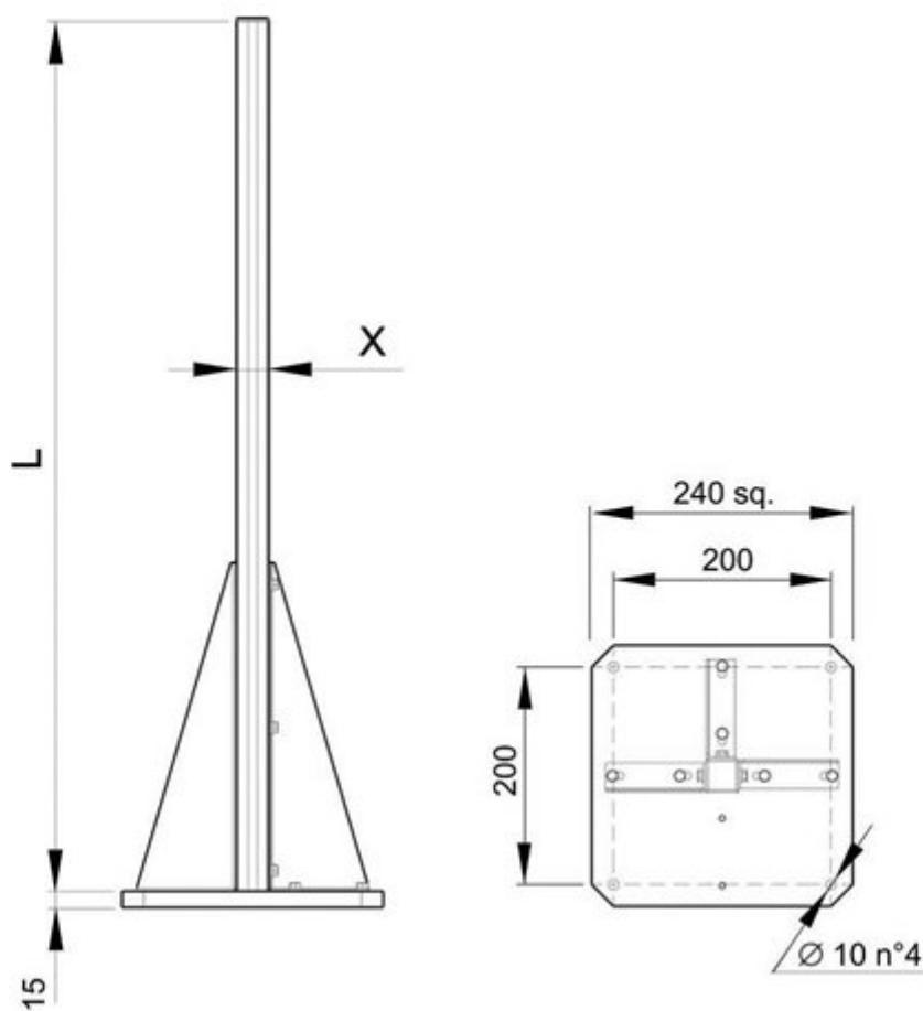
Fig 93 - Dimensions (mm)
