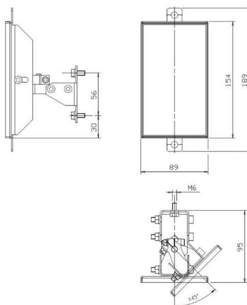
Fig 95 - SG-DM 150 Dimensions (mm)
