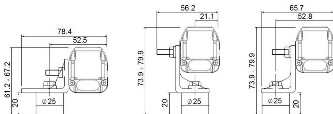
Fig 87 - Angled fixing bracket + Antivibration support
