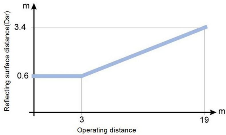
Fig 14 - Minimum distance from reflective surface
