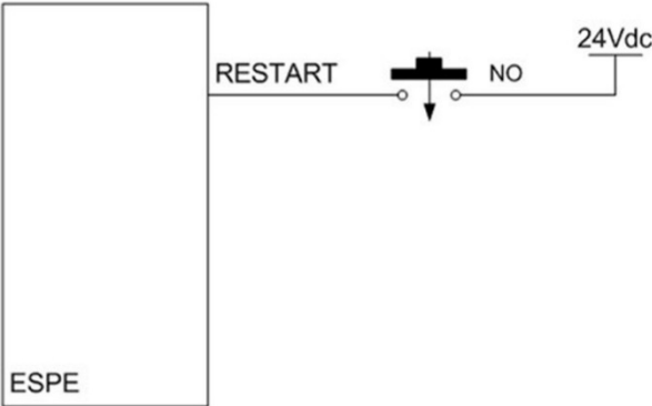
Fig 44 - Restart connection (manual)
