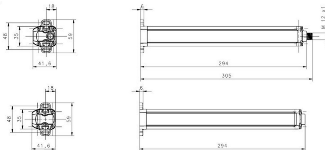
Fig 109 - Dimensions (mm)
