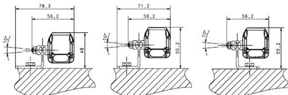
Fig 81 - Angled fixing bracket + Orientable support
