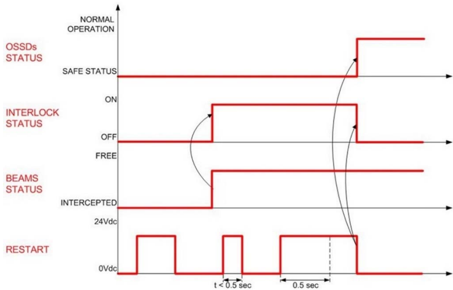
Fig 43 - Restart timings (manual)
