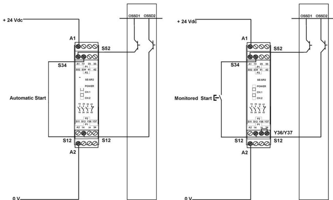
Fig 31 - Connection to SE-SR2 Safety Relais
