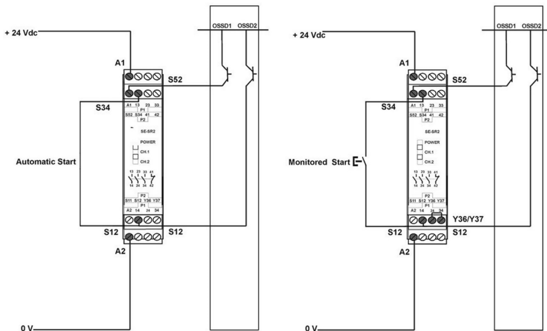
Fig 102 - Safety relay
