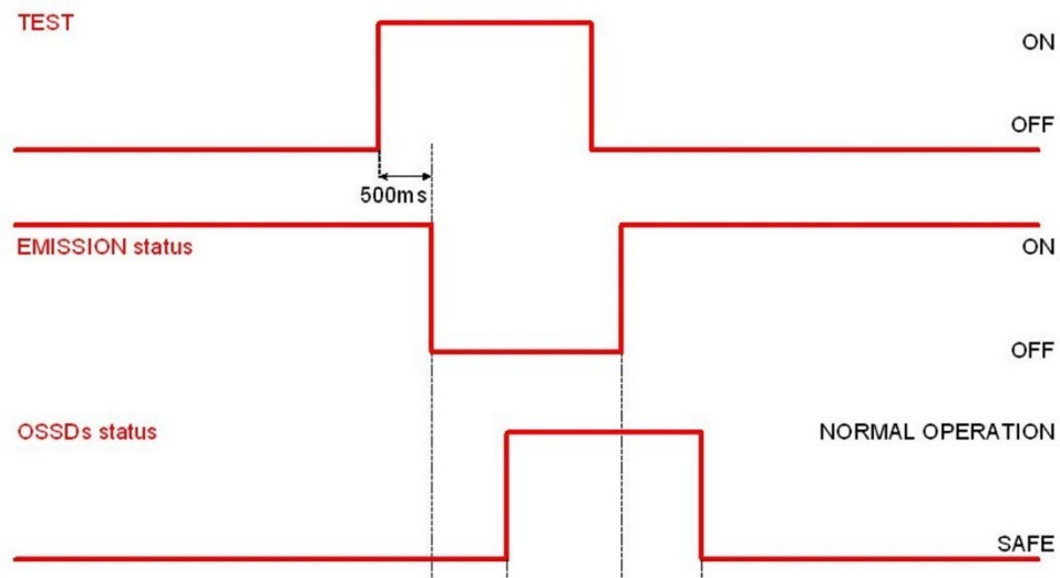
Fig 46 - Test timings
