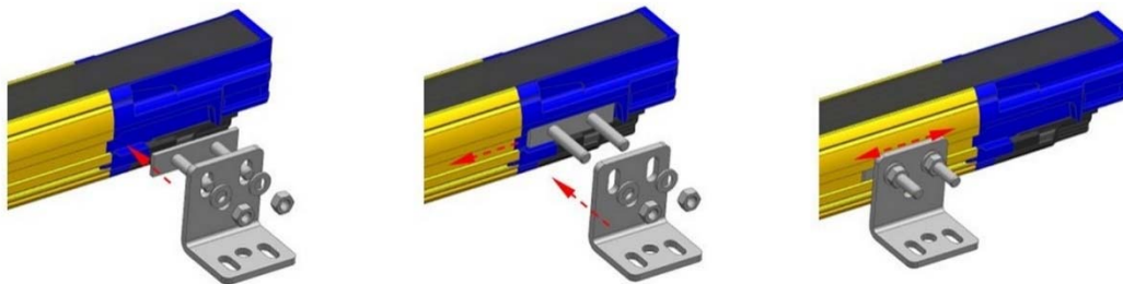
Fig 21 - Fixed brackets mounting procedure
