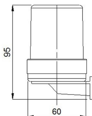
Fig 104 - Lamp LMS
