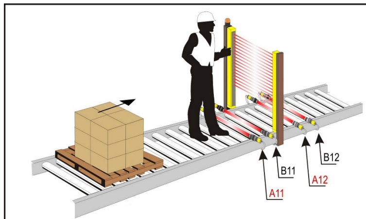
Fig 57 - Typical Muting Application
