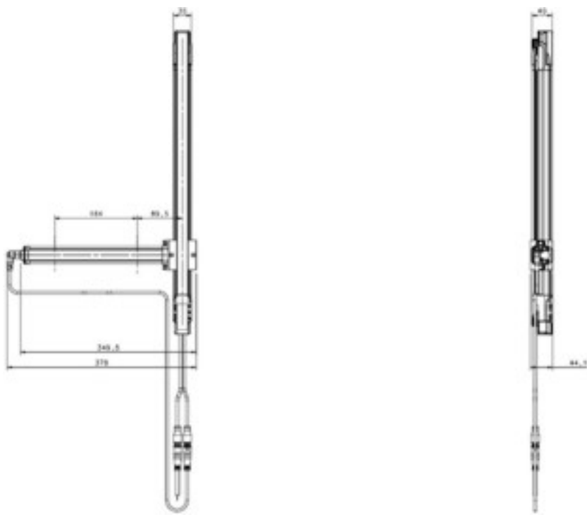
Fig 113 - Light curtain + Active/Passive arms L
