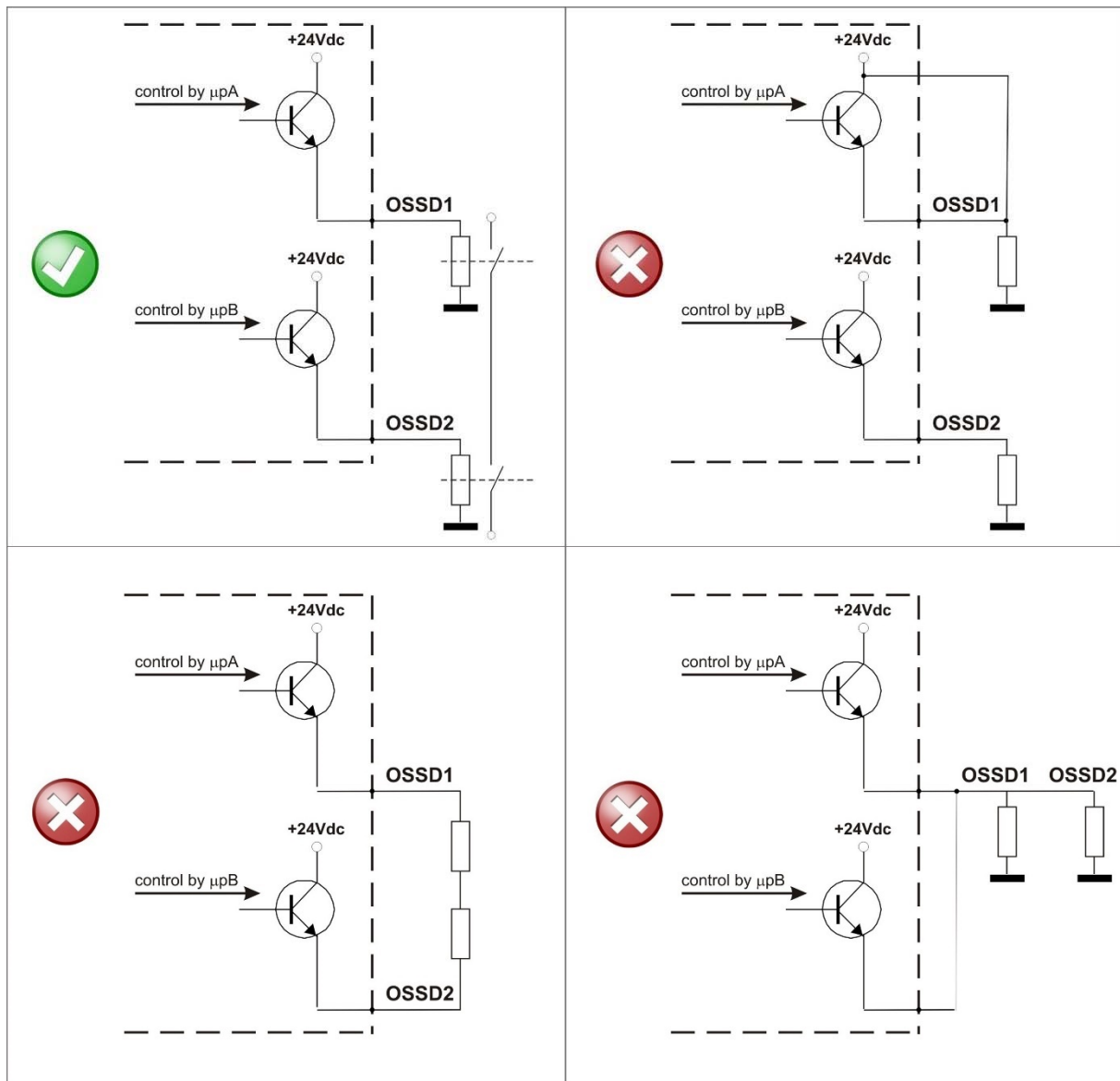
Fig 32 - OSSDs connection
