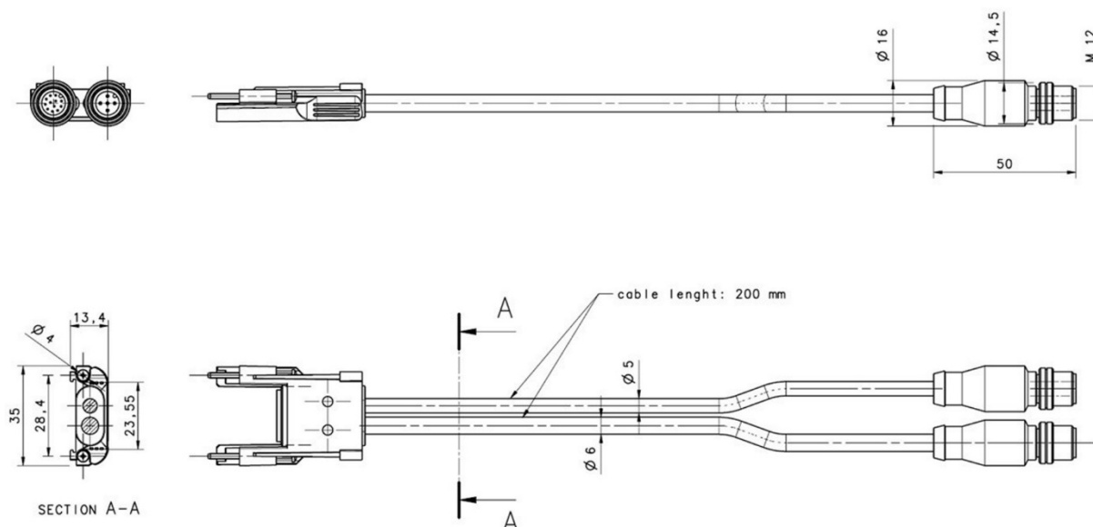
Fig 99 - RX MUTING - Pigtail cable
