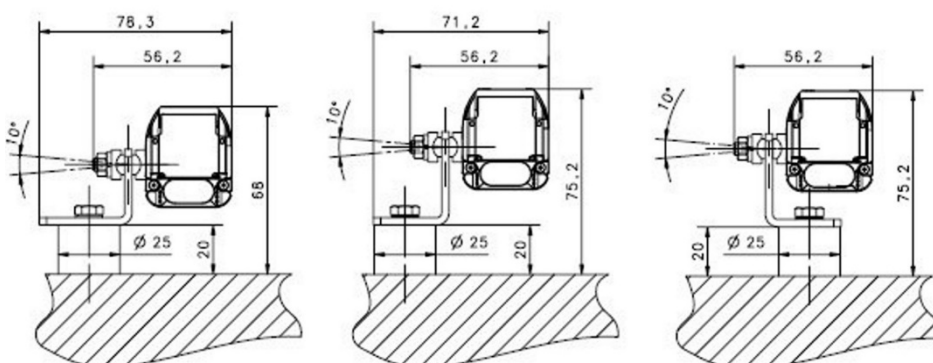
Fig 83 - Angled fixing bracket + Orientable support + Antivibration support
