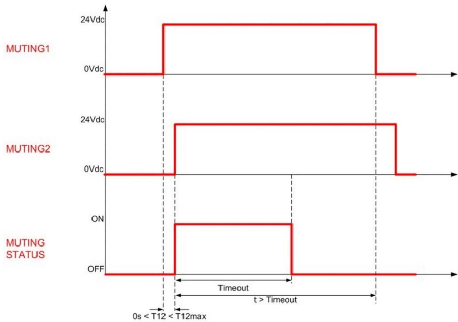
Fig 63 - Muting timeout
