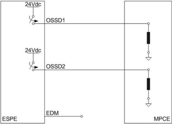
Fig 50 - EDM connection (PNP configuration)
