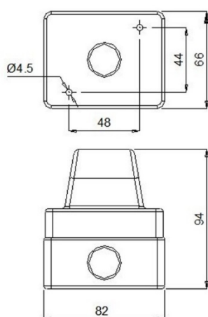
Fig 104 - Lamp LMS
