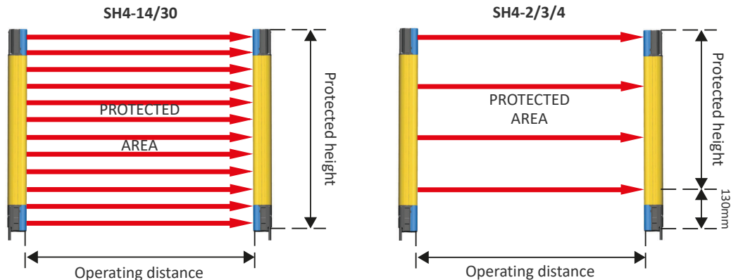
Figure 2: Detection zone
