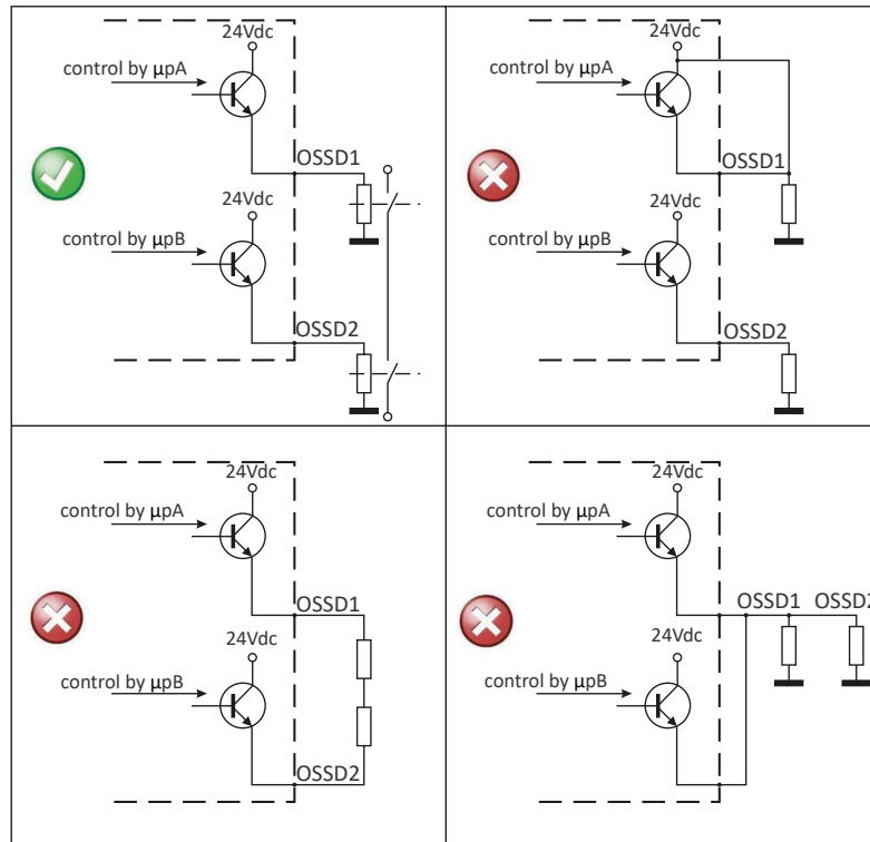
Figure 25: OSSDs connection
