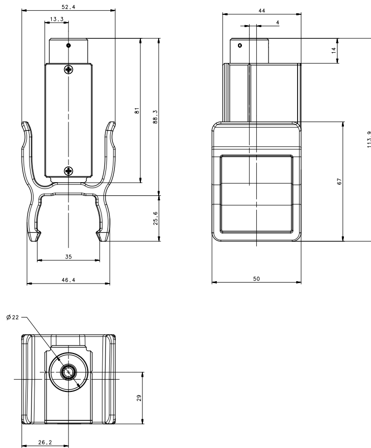
Figure 76 - Dimensions (mm)
