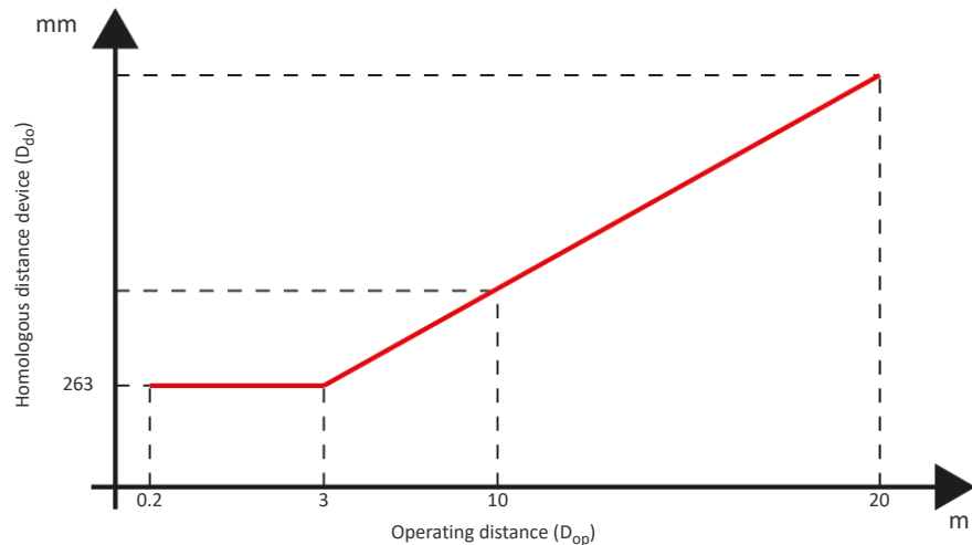
Figure 12 - ESPE Type 4
