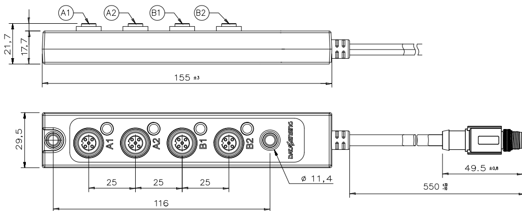
Figure 87 - Dimensions (mm)
