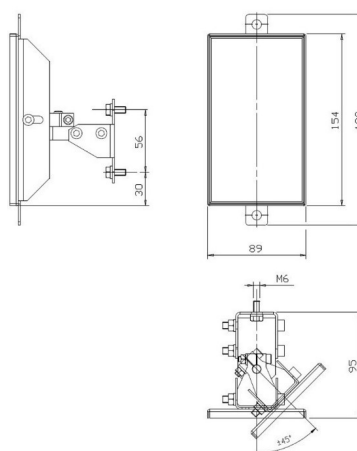
Figure 73 - SG-DM 150 (mm)
