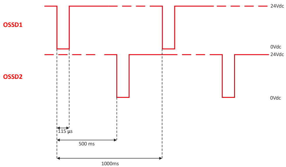
Figure 26: Behavior of OSSDs
