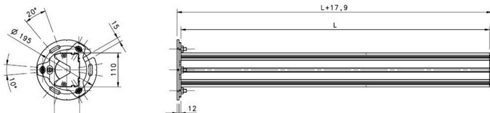
Figure 67 - Protective Stands
