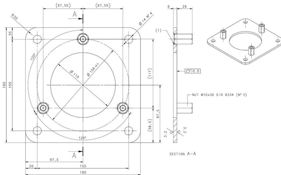
Figure 69 - Plate kit
