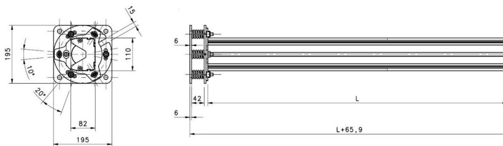
Figure 70 - Mounting with SG-P SB
