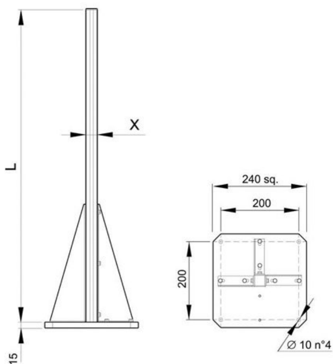
Figure 71 - Dimensions (mm)
