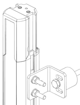
Figure 22: Anti-vibration dampers
