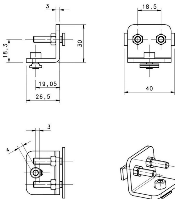
Figure 68 - Mounting kit
